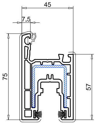
Hoja deslizante 75 mm ref. 105.322 Refuerzo 113.034.2 Refuerzo 113.031.2
