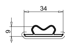
Tapa lateral ref. 109.635 para 105.322/327
