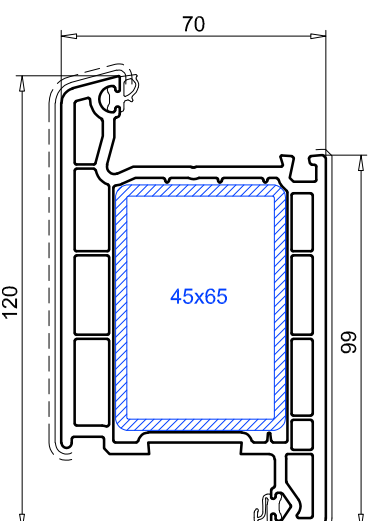
Hoja SL70, 120 mm ref. 105.232 Refuerzo 113.286.3 Tope soldable 141.520
