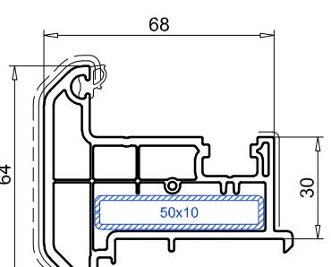
Batiente SL70, 64 mm ref. 102.236 Refuerzo 113.013 Remate 109.524 Remate 109.508.1
