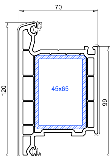
Hoja SL70, 120 mm ap. exterior ref. 105.233 Refuerzo 113.286.3 Tope soldable 141.520
