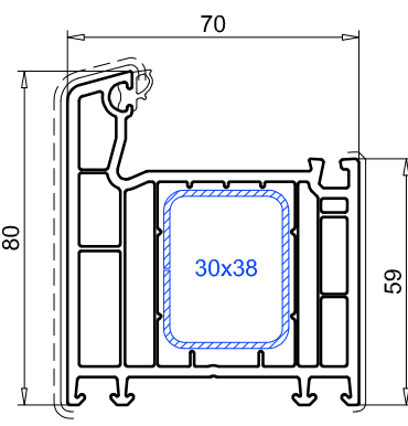
Marco SL70, 80 mm ref. 101.214 Refuerzo 113.271
