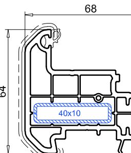
Batiente acilpsado SL70, 64 mm ref. 102.234 Refuerzo 113.028 Remate 1 pieza 109.598 Remate 2 piezas 109.600
