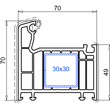
Marco SL70, 70 mm ref. 101.226 Refuerzo 113.025
