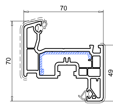
Hoja SL70, 70 mm ref. 103.229 Refuerzo 113.269
