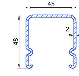
Refuerzo hojas ref. 113.368.2 Para hojas 103.241/242/273
