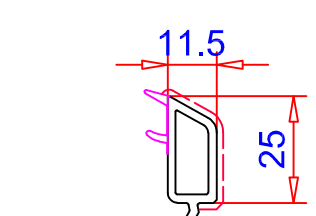
Junquillo 11.5mm Ref. 107.262 para 42 mm
