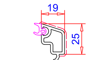
Junquillo 19.0mm Ref. 107.277 Vidrio 33/ 34/ 35 mm
