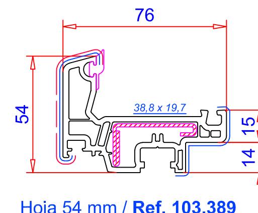
Hoja 54 mm / Ref. 103.389 Refuerzo: 113.363 Remates: 109.667
