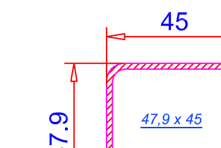
Refuerzo 47,9 x 45,0 mm Ref. 113.368.2 para 103.385 / 103.386
