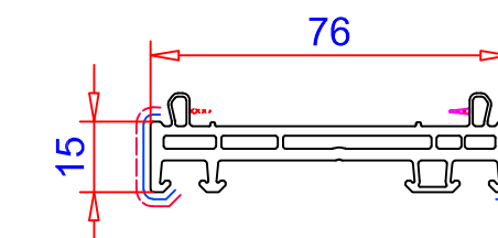
Ensanche 15 mm Ref. 114.052
