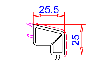
Junquillo 25.5mm Ref. 107.274 Vidrio 28 mm
