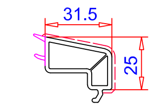
Junquillo 31.5mm Ref. 107.270 Vidrio 22 mm
