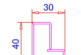
Refuerzo 40,0 x 30,0 mm Ref. 113.367 para 101.351 / 101.354
