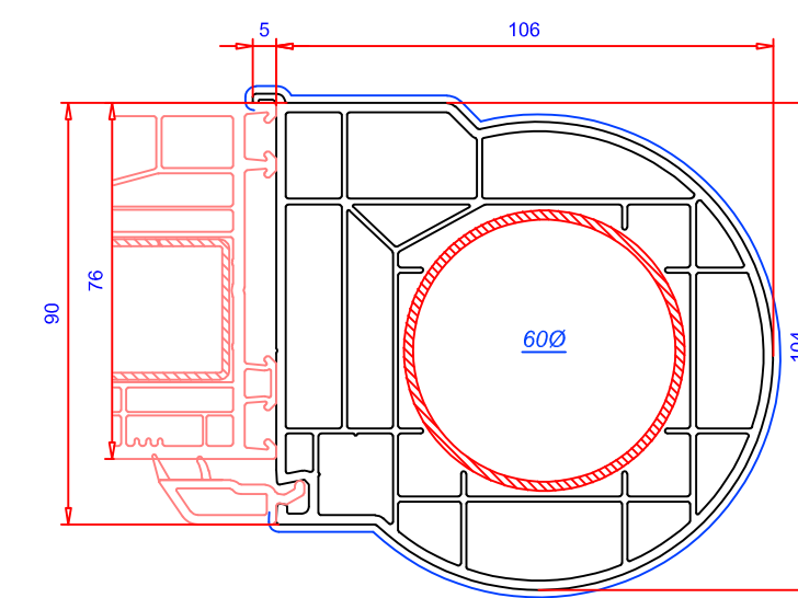
Esquinero regulable 106 x 90 mm Ref. 116.216.2 Junquillo 107.261 Refuerzo: 113.054.2
