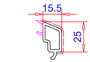
Junquillo 15.5mm Ref. 107.264 Vidrio 38 mm
