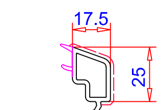
Junquillo 17.5mm Ref. 107.265 Vidrio 36 mm
