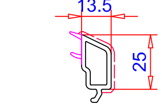
Junquillo 13.5mm Ref. 107.263 Vidrio 40 mm
