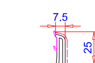
Junquillo 7.5mm Ref. 107.278 Vidrio 48 mm
