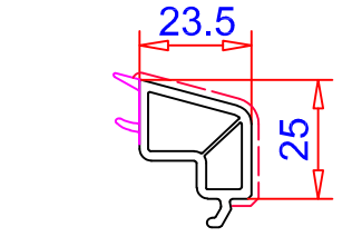
Junquillo 23.5mm Ref. 107.268 Vidrio 30 mm
