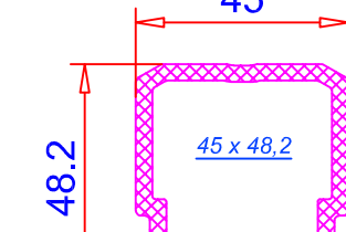
Refuerzo alu. 45,0 x 48,2 mm Ref. 115.003 para 103.385 / 103.386
