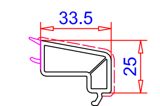
Junquillo 33.5mm Ref. 107.272 Vidrio 20 mm
