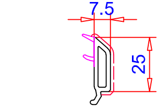
Juquillo 7.5mm Ref. 107.260 Vidrio 46 mm
