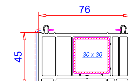
Ensanche 45 mm Ref. 114.054 Refuerzos: 113.025 / 113.025.2 / 113.025.3
