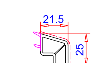
Junquillo 21.5mm Ref. 107.267 Vidrio 32 mm
