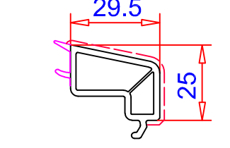
Junquillo 29.5mm Ref. 107.273 Vidrio 24 mm
