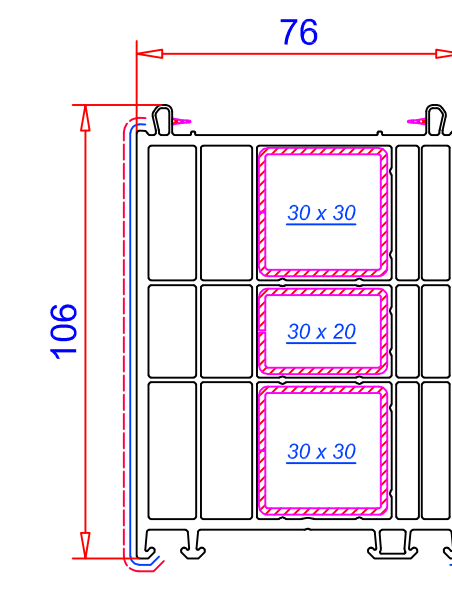
Ensanche 100 mm Ref. 114.055 Refuerzos: 113.025 / 113.025.2 / 113.025.3 / 113.019
