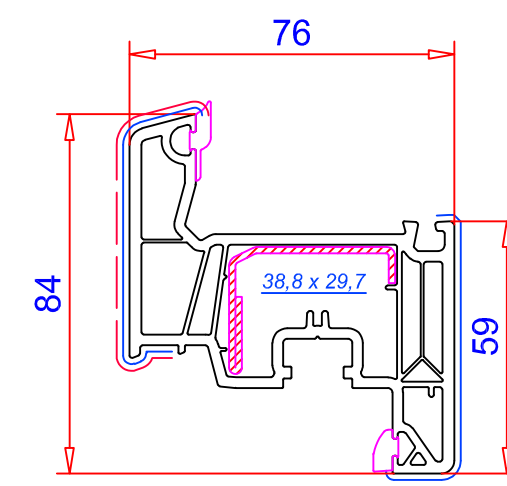
Hoja 84 mm / Ref. 103.381 Refuerzos: 113.292 113.294.2 / 113.295 / 113.394.2
