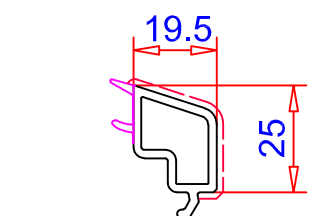
Junquillo 19.5mm Ref. 107.266 Vidrio 34 mm
