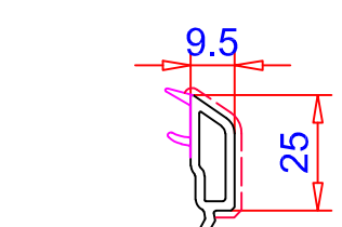
Junquillo 9.5mm Ref. 107.261 Vidrio 44 mm
