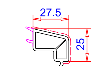
Junquillo 27.5mm Ref. 107.269 Vidrio 26 mm
