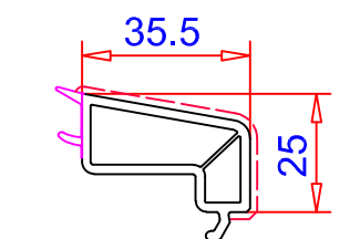
Junquillo 35.5mm Ref. 107.271 Vidrio 18 mm
