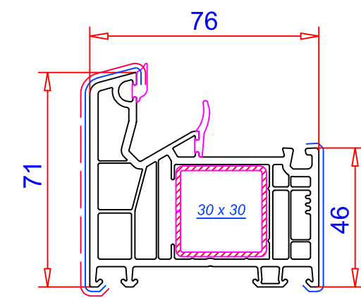
Marco JC 71mm / Ref. 101.350 Refuerzos: 113.025 / 113.025.2 / 113.025.3
